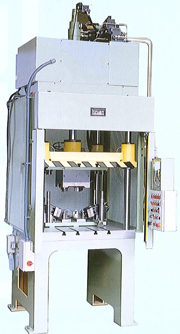
Open gap and four columned hydraulic presses.
